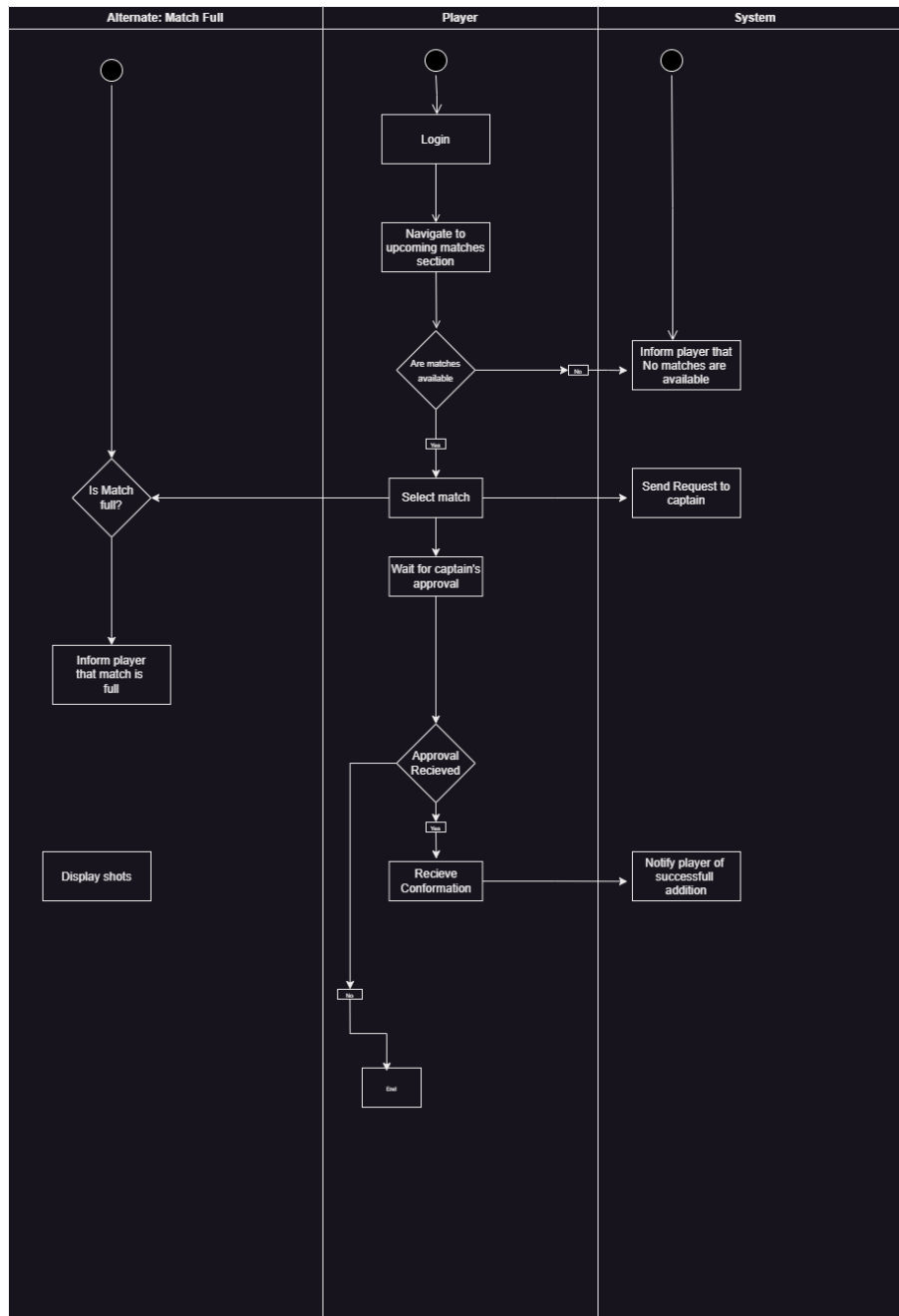
Figure 3.20: Activity diagram for Join Match
