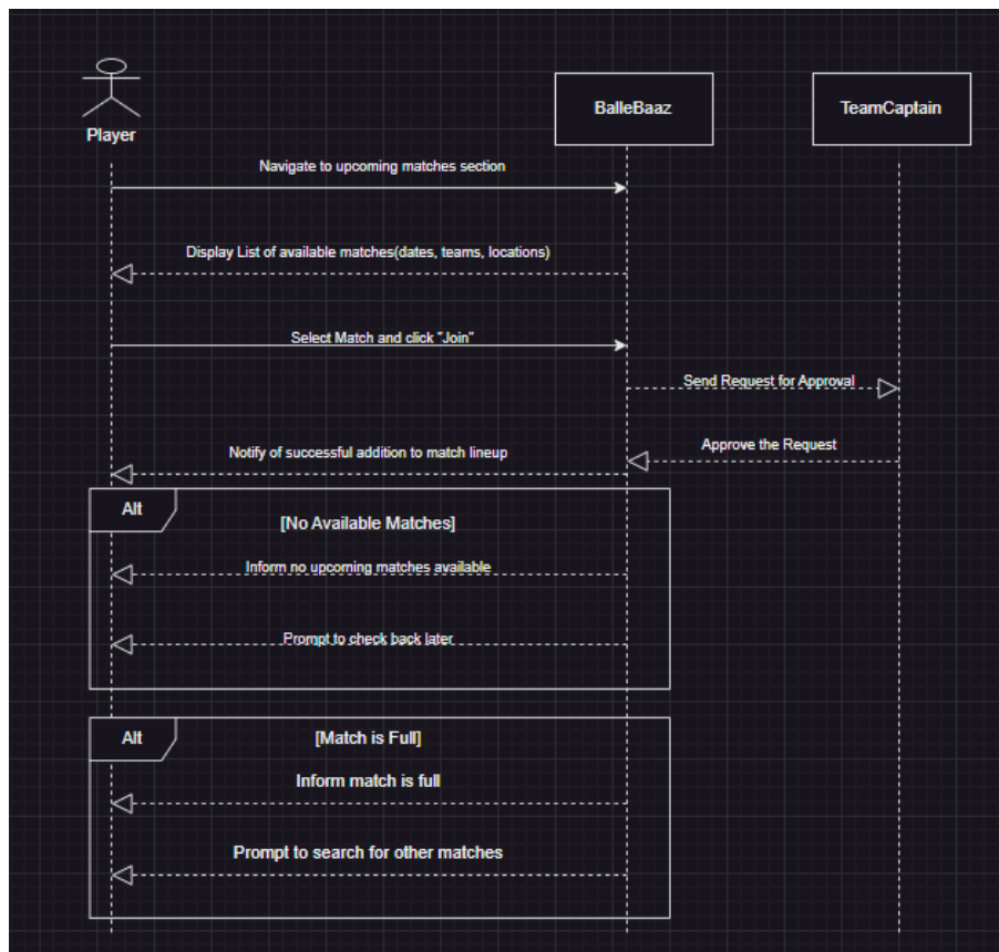
Figure 3.3: Sequence Diagram for Player Join Match
