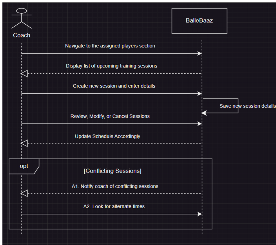
Figure 3.17: Sequence Diagram for Coach Manage Sessions
