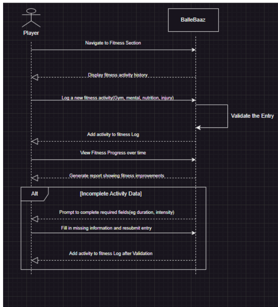
Figure 3.4: Sequence Diagram for Player Track Fitness
