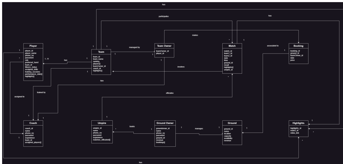
Figure 2.2: Domain Model of BalleBaaz
