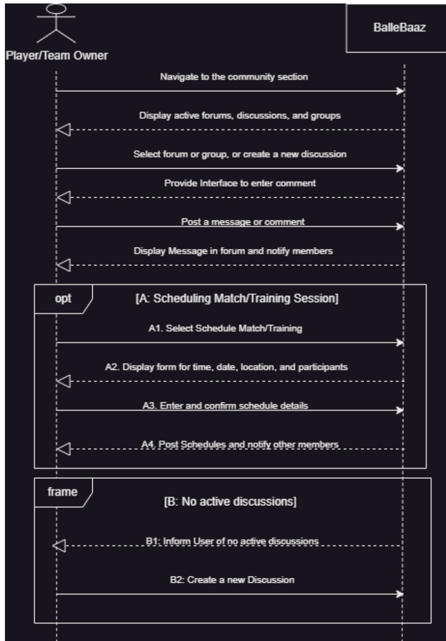
Figure 3.18: Sequence Diagram for Community Interactions
