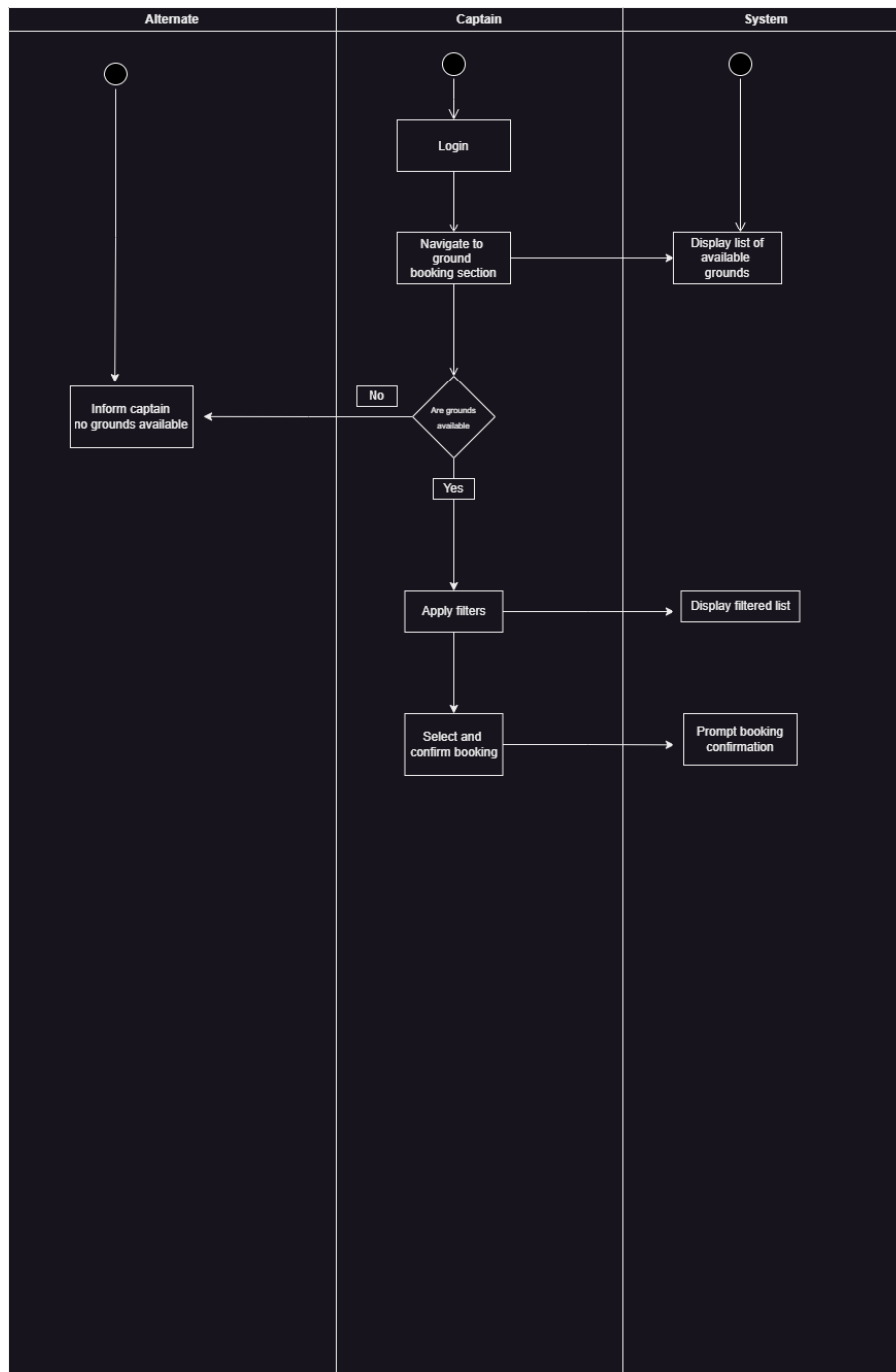
Figure 3.27: Activity diagram for Captain ground booking
