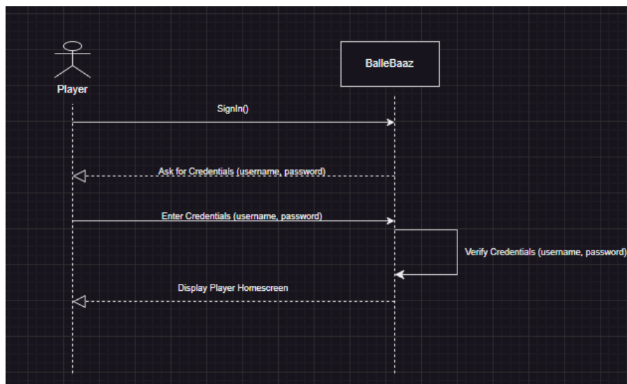
Figure 3.2: Sequence Diagram for Player Sign In
