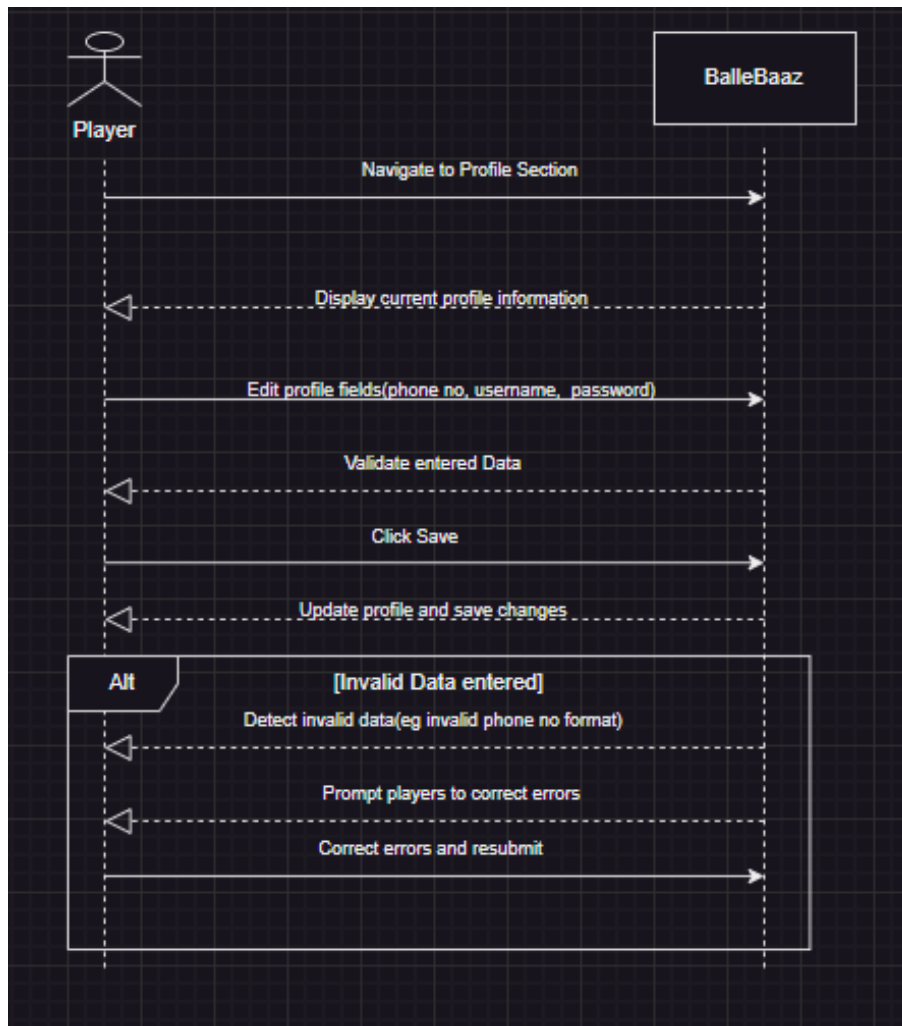
Figure 3.5: Sequence Diagram for Player Modify Profile
