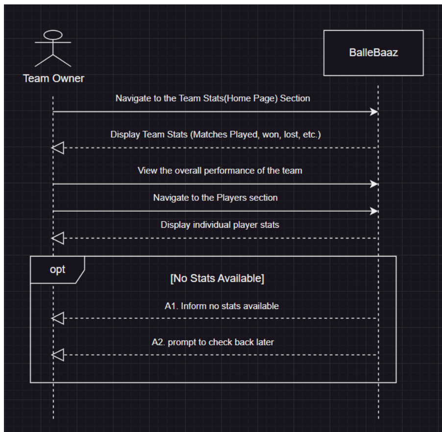
Figure 3.13: Sequence Diagram for Team Owner Analyze Stats
