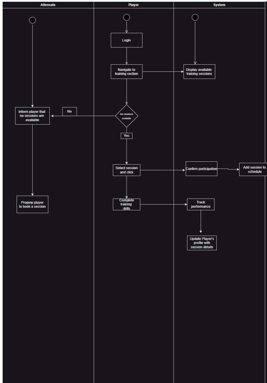
Figure 3.22: Activity diagram for Training Session
