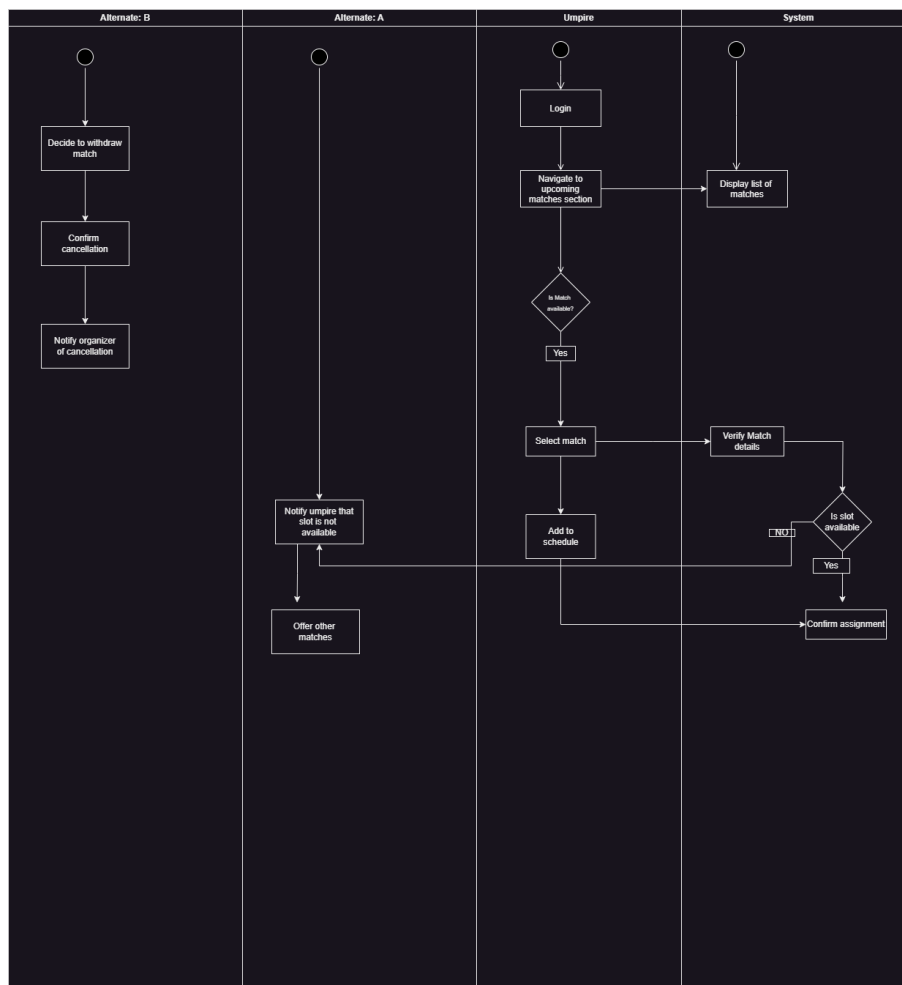
Figure 3.24: Activity diagram for Upcoming Matches
