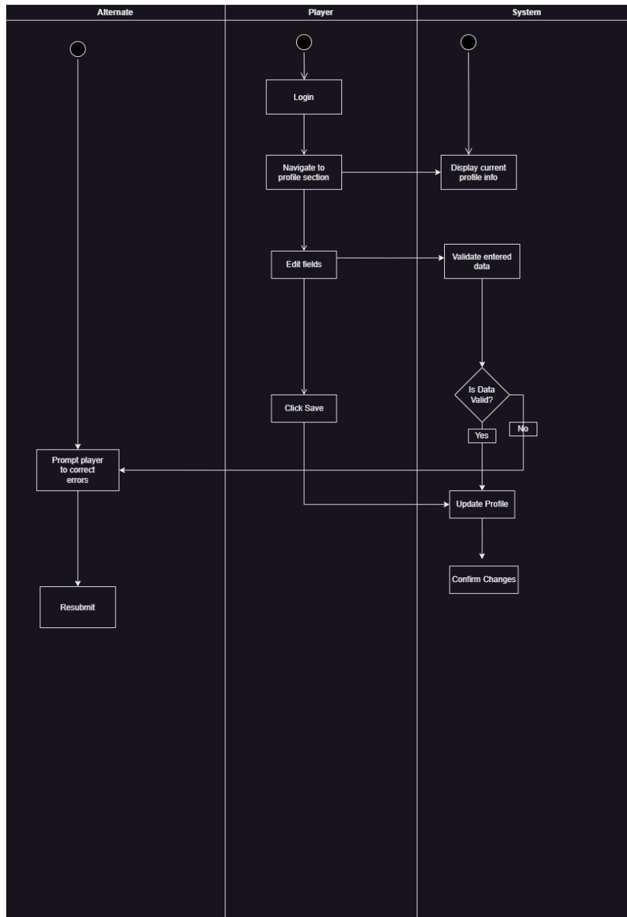
Figure 3.21: Activity diagram for Manage profile
