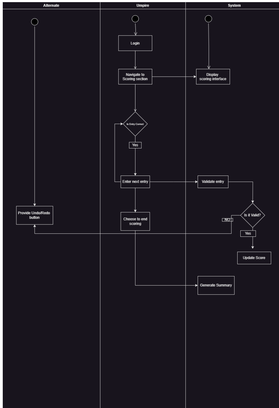
Figure 3.23: Activity diagram for Scoring
