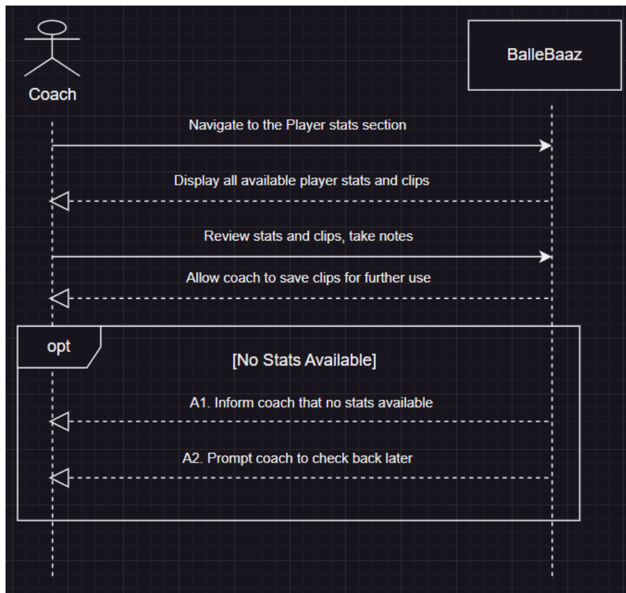
Figure 3.16: Sequence Diagram for Coach Review Stats
