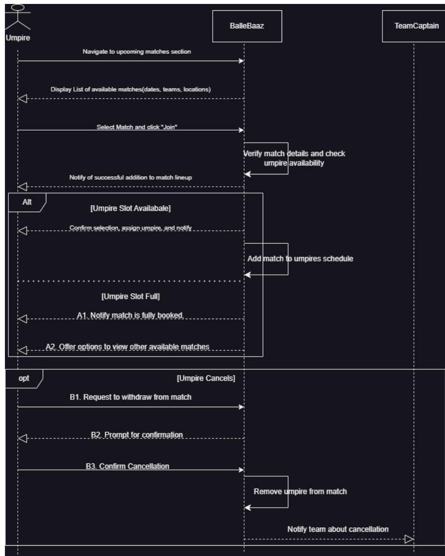
Figure 3.9: Sequence Diagram for Umpire Officiate Match
