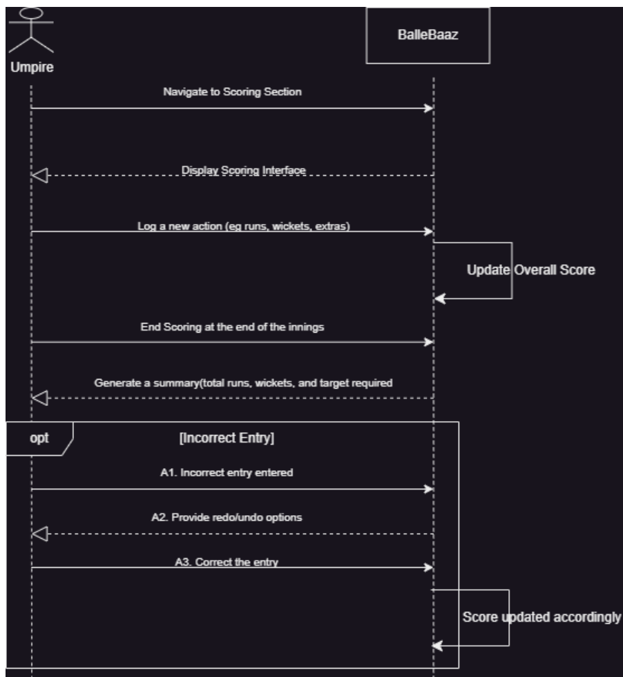
Figure 3.11: Sequence Diagram for Umpire Do Scoring
