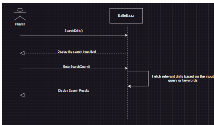
Figure 3.7: Sequence Diagram for Player Search Drills
