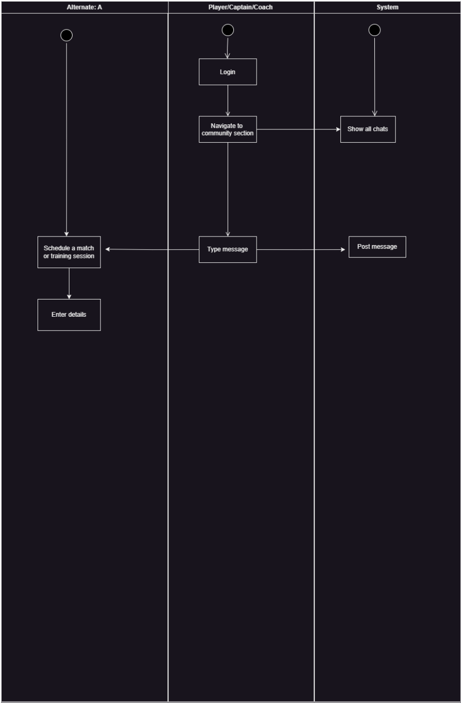
Figure 3.31: Activity diagram for Community Section
