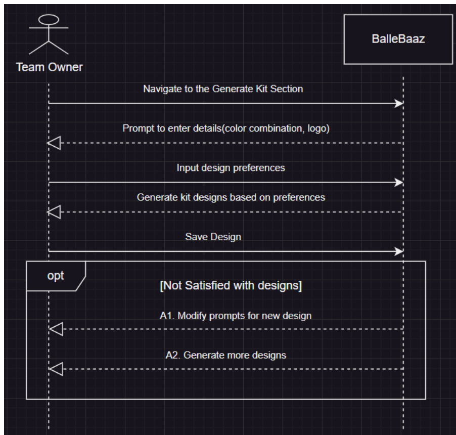
Figure 3.15: Sequence Diagram for Team Owner Generate Kit Design
