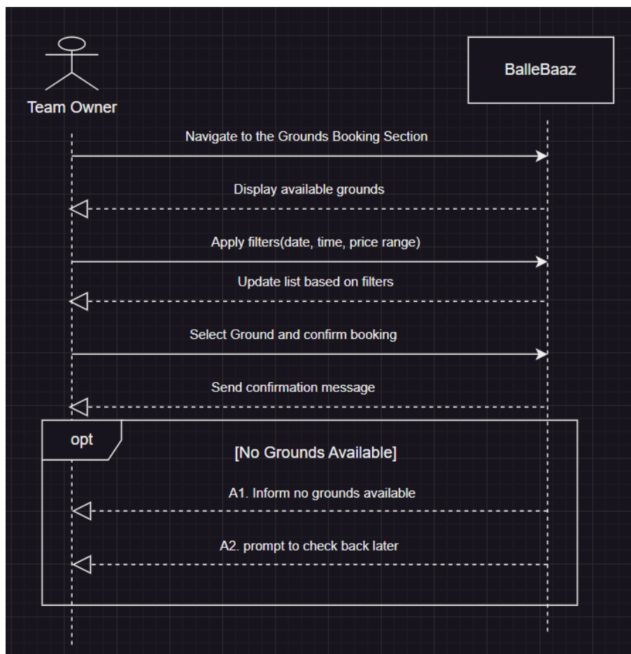
Figure 3.14: Sequence Diagram for Team Owner Book Ground
