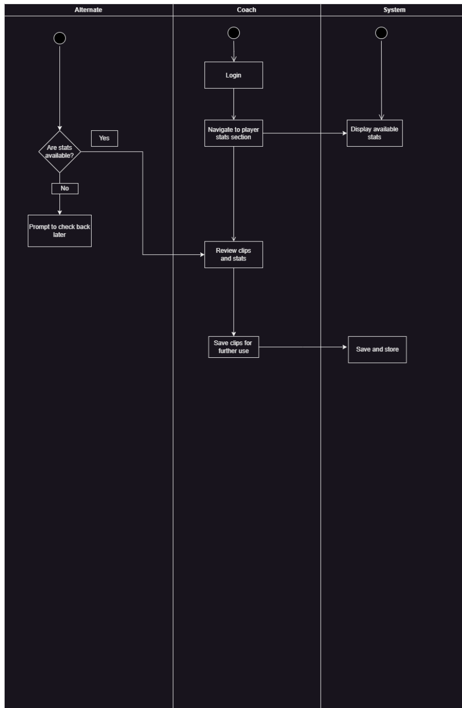
Figure 3.29: Activity diagram for Coach review stats
