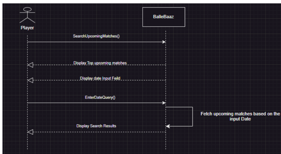
Figure 3.8: Sequence Diagram for Player Search Upcoming Matches
