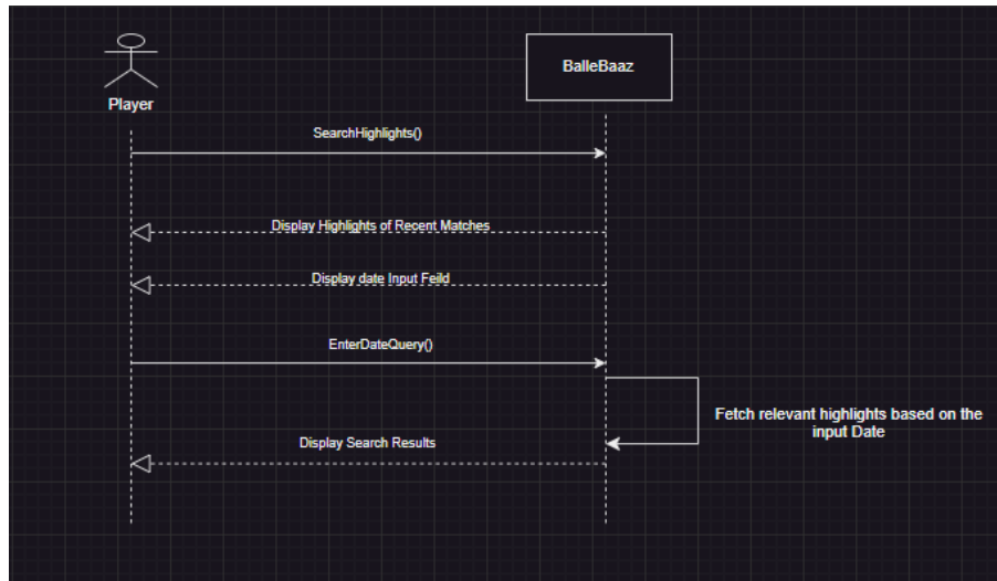
Figure 3.6: Sequence Diagram for Player Search Highlights
