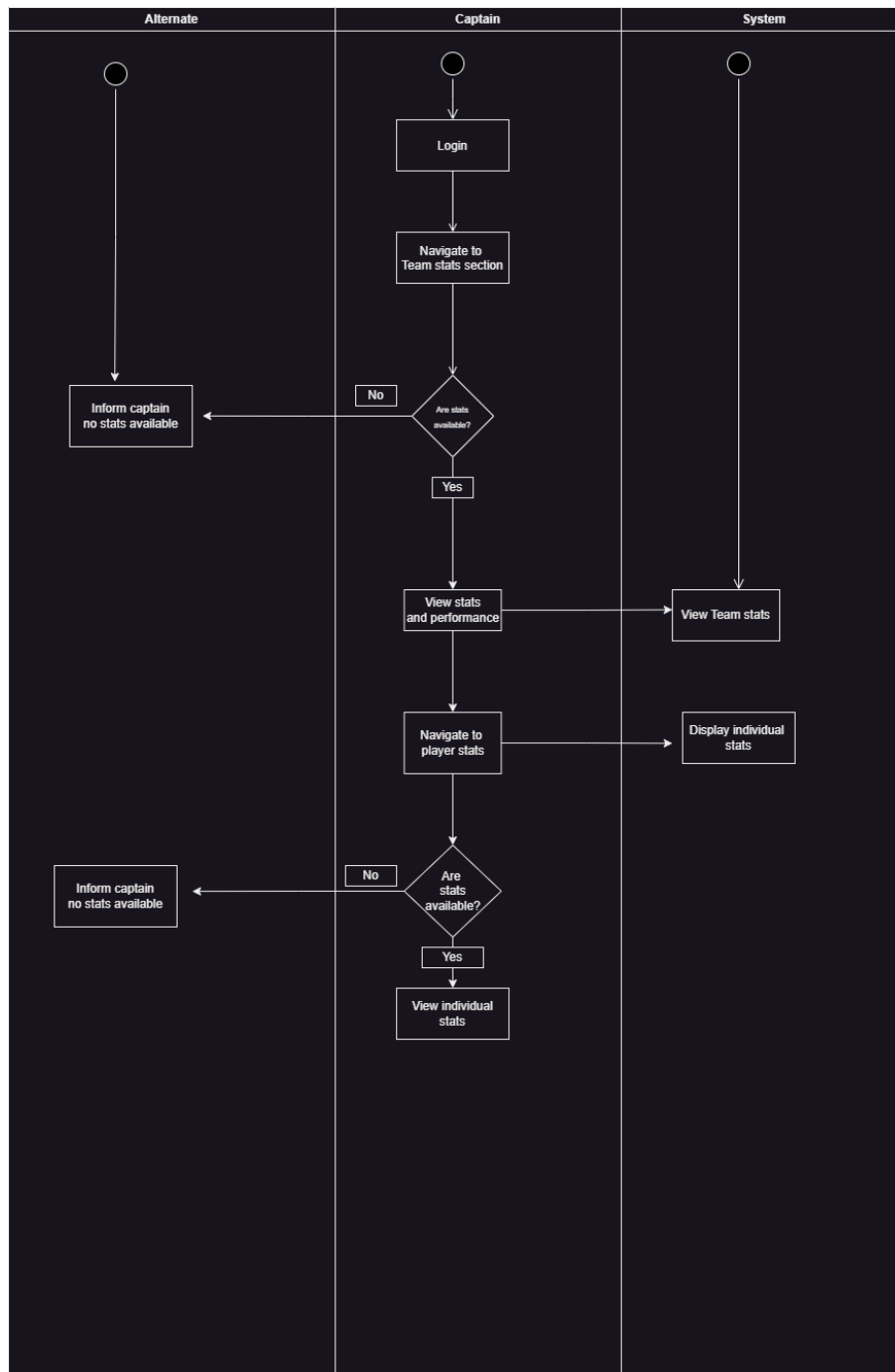
Figure 3.26: Activity diagram for Analyze Stats
