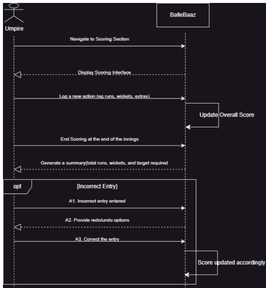
Figure 3.10: Sequence Diagram for Umpire Do Scoring
