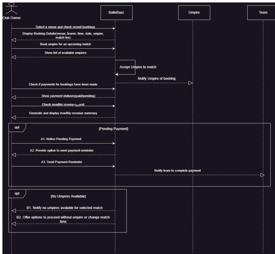
Figure 3.12: Sequence Diagram for Club Owner
