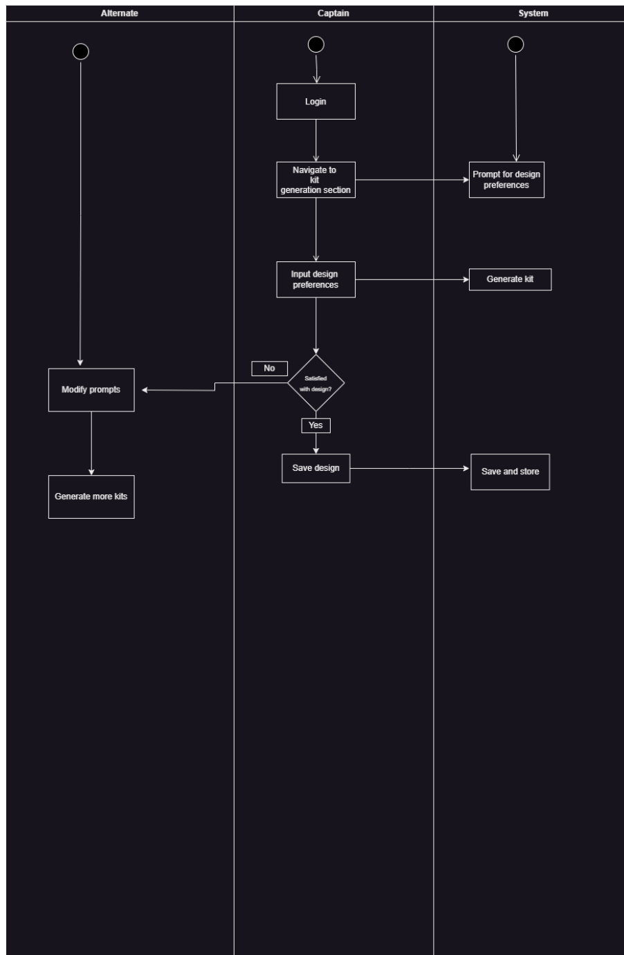
Figure 3.28: Activity diagram for Kit Generation
