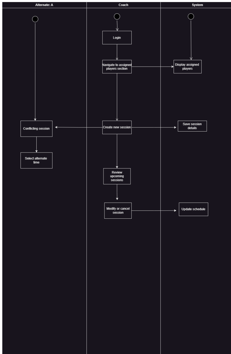
Figure 3.30: Activity diagram for Coach assigned players
